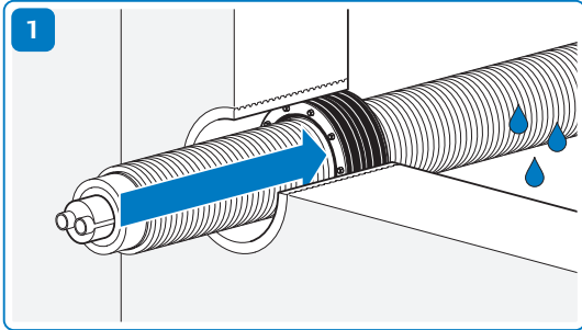
1 Insert the PWP wall seal as far as the water side (outside) – nuts face the cellar side
