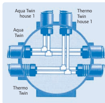
Heating and tap water from the main lines to the house
