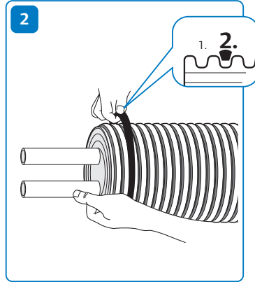
2 Install the rubber seal in the second groove.
