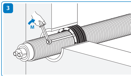
3 During final assembly, successively tighten up each nut with torque-wrench clockwise until the maximum torque M_{max} is reached. Tighten the nuts several times. Repeat the procedure after two hours.
