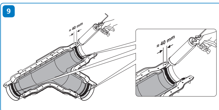
Apply sealant to spacer pieces.
