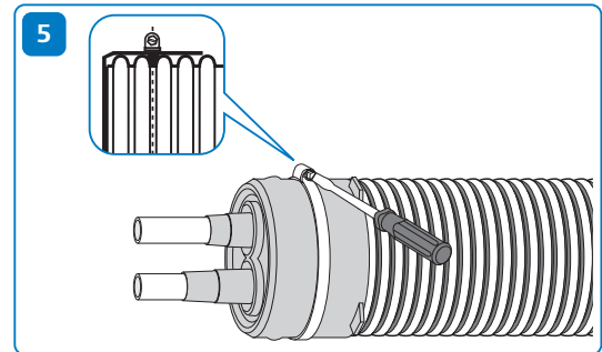
5 Position the jubilee clip over the seal and tighten.
