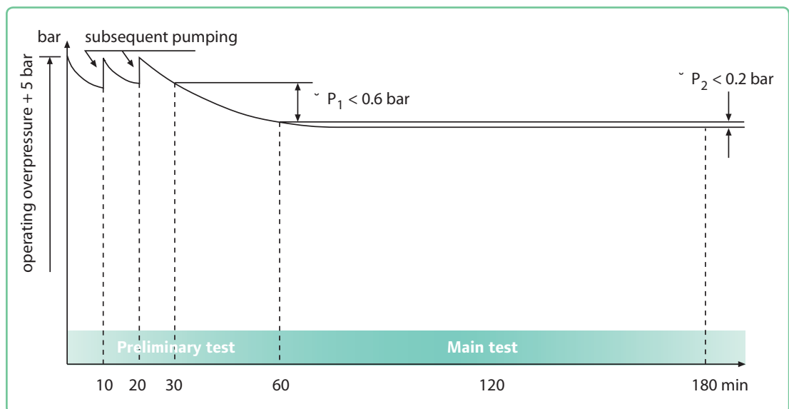
Pressure test diagram
