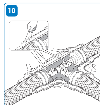
Partially release adhesive strips.
