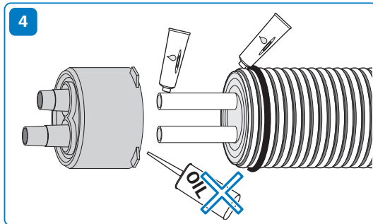
4 Install the end cap over the end of the pipe using lubricant. A non oil-based lubricant can assist.
