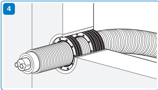
4 Use Uponor PWP supplementary set to reduce tension
