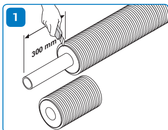
1 Cut back outer jacket.
