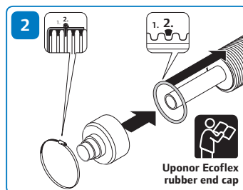
2 Fit rubber end cap.
