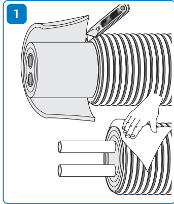
1 Cut away jacket pipe and peel off insulation layers so that enough flow pipe is visible to join the coupling and the end cap. Be careful not to damage the flow pipe. Clean the surfaces carefully.
