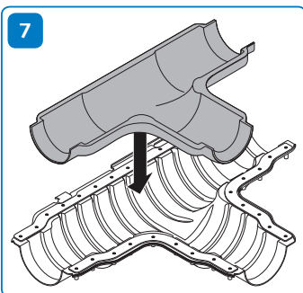
Place foam half-shell in casing.
