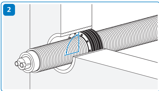
2 Install Uponor PWP wall seal pipe at right angles to Uponor pipe
